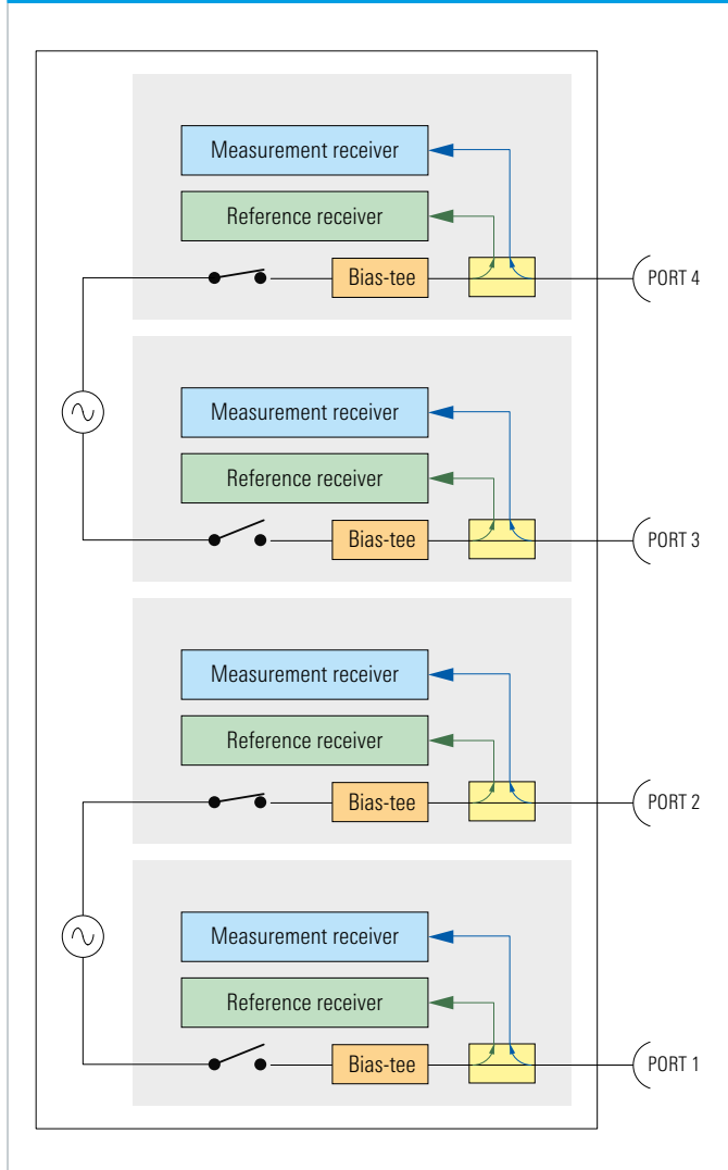
Block diagram for R&S®ZVA four-port model
