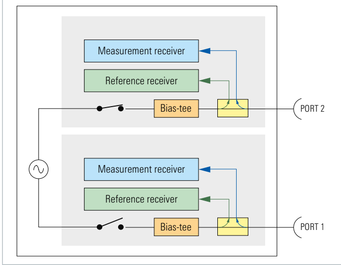
Block diagram for R&S®ZVA two-port model
