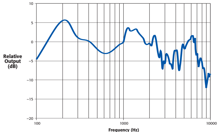
Figure 4. Frequency Response
