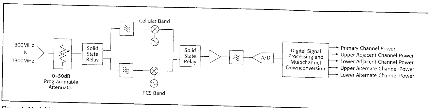
Figure 1. Model 2800 Front End Block Diagram. A unique signal processing configuration generates up to five power measurements in five different frequency bands simultaneously.
