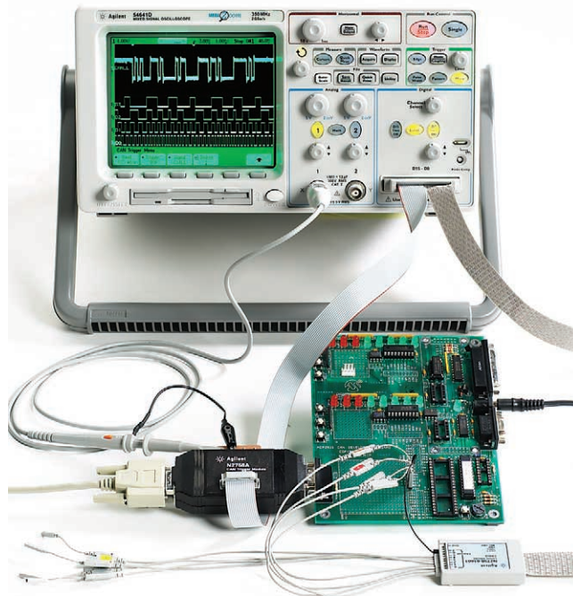
The N2758A CAN trigger module reduces the time required to debug your mixed signal CAN based designs.
