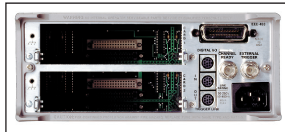
Model 7001 rear panel
