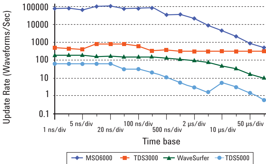
Comparison of waveform update rates using each scope's default real-time acquisition mode.
