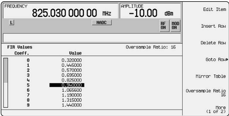
Implement custom FIR filters via the FIR table editor.
