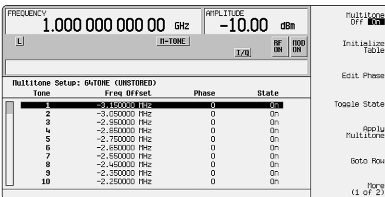
Multitone editor setup.
