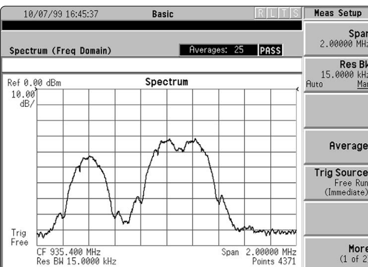
Multicarrier GSM spectrum resulting from the configuration shown in GSM setup.
