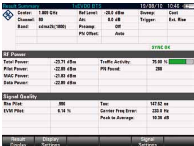
Analysis of a 1xEV-DO transmit signal.
