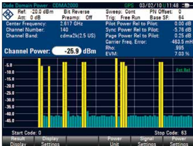
The code domain power measurement provides an overview of the key signal parameters.
