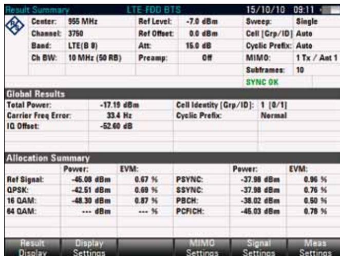
Analysis of an LTE FDD transmit signal.
