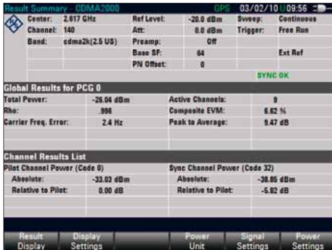
Analysis of a CDMA2000® transmit signal with the R&S®FSH-K46 option.
