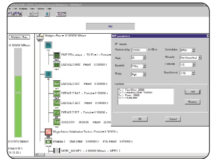
► Figure 9. Custom transport stream with Mega-frame.
