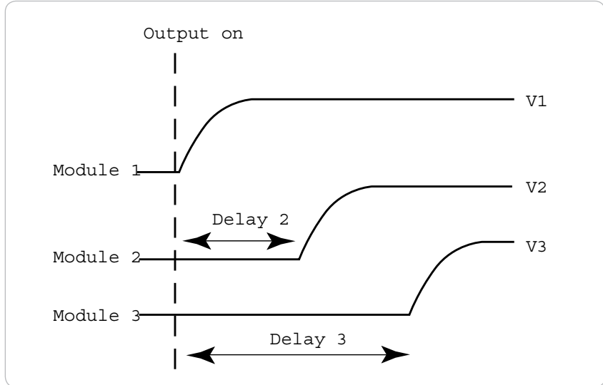
Figure 2. Output sequencing
