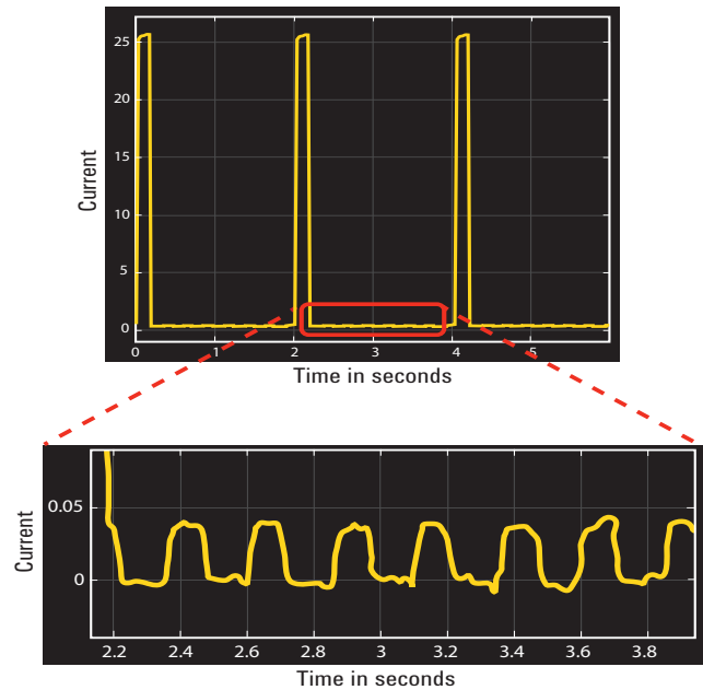
Figure 1. Dynamic current measurement
