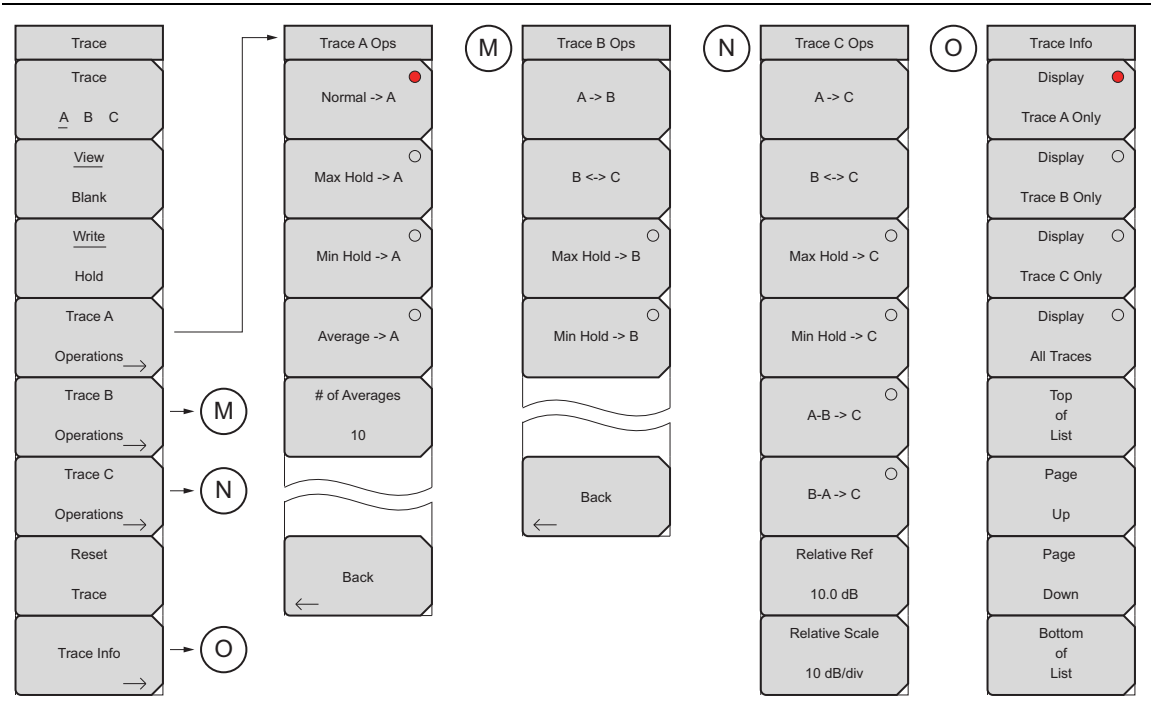
Figure 2-32. Trace Submenu Keys
