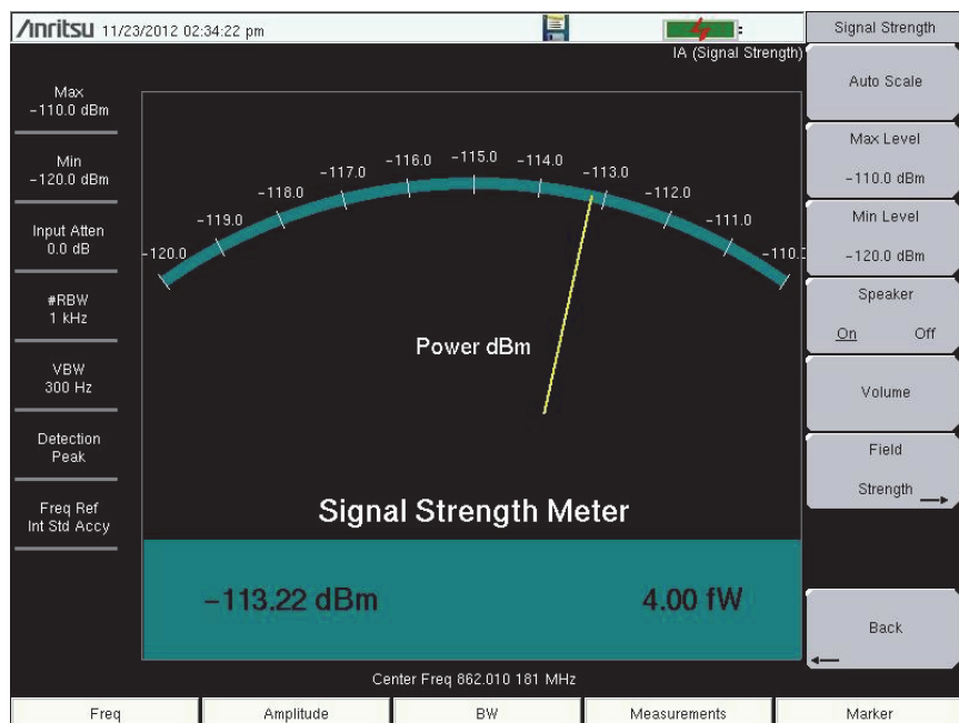
Figure 3-2. Interference Analyzer Signal Strength
