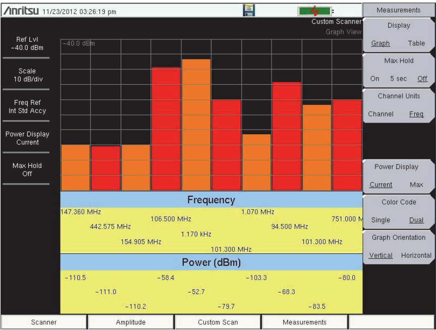
Figure 4-9. Channel Scanner Graph Display with Vertical Orientation
