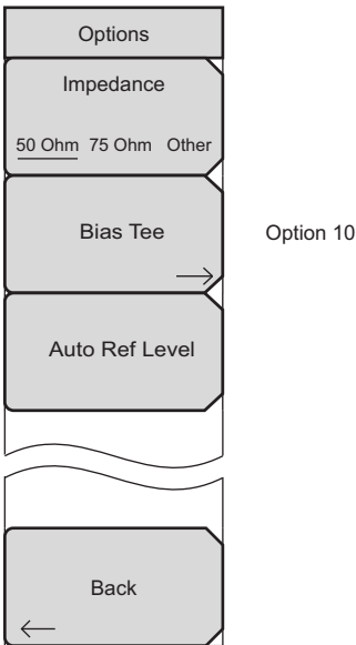
Figure 2-34. System Menu, Application Options Submenu Keys
