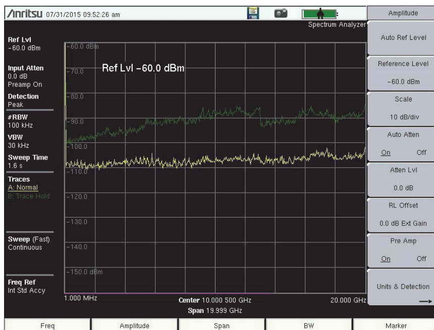
Figure 2-9. Preamplifier On and Off
