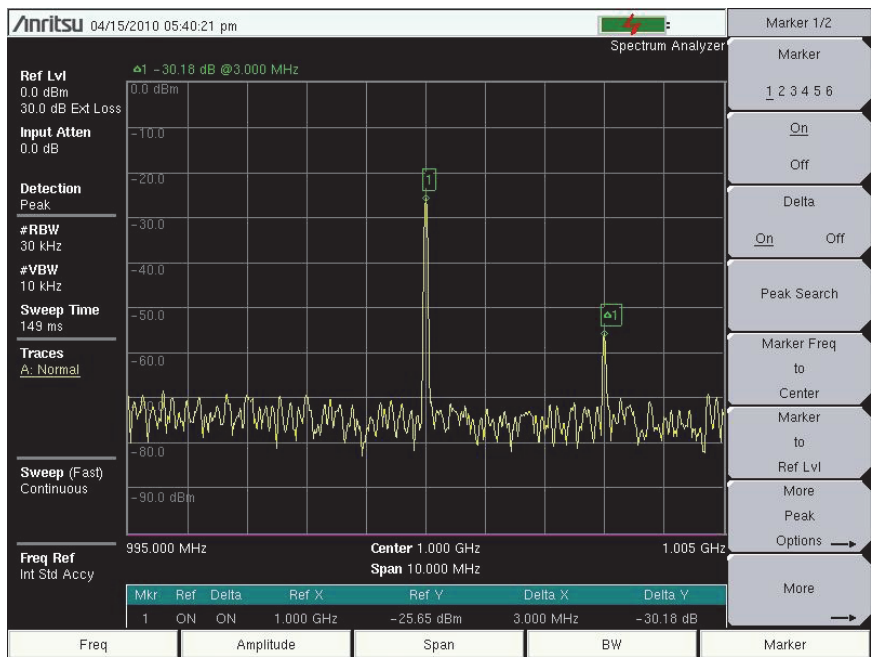
Figure 2-12. Out-of-Band Spurious Emission Measurement
