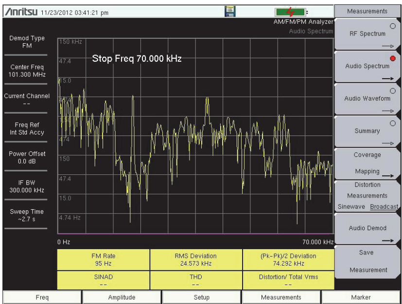
Figure 7-1. Audio Spectrum
