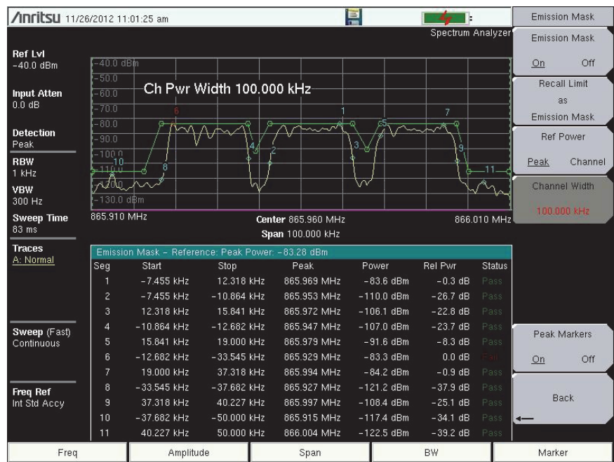
Figure 2-16. Emission Mask (In-Band)
