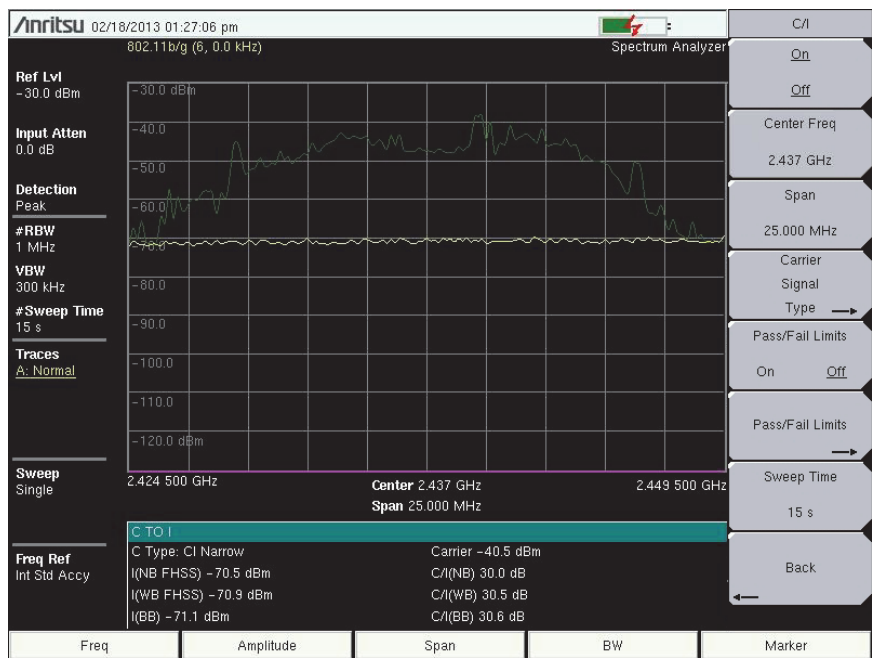
Figure 2-15. C/I Measurement, Results
