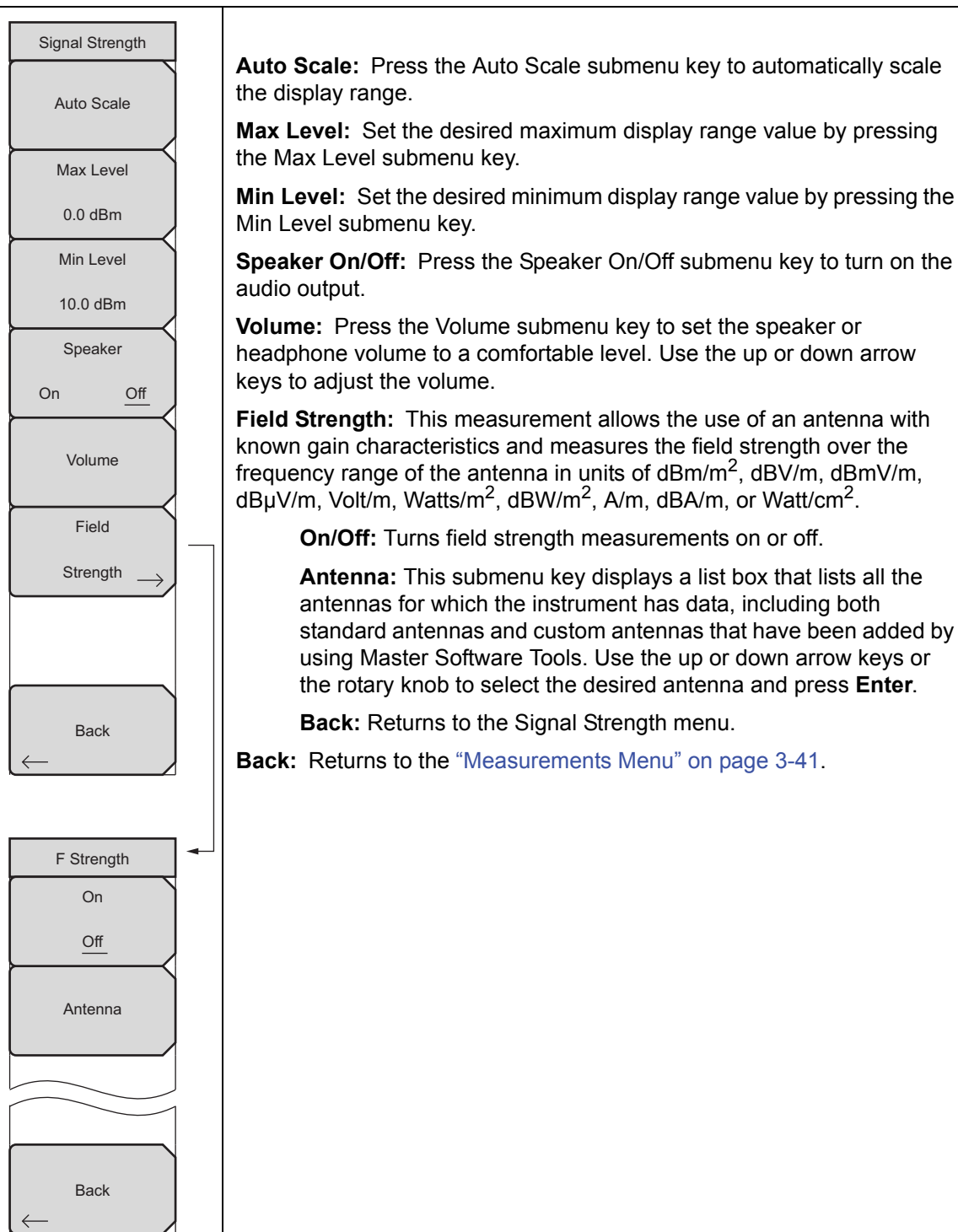
Figure 3-58. IA Signal Strength Menu
