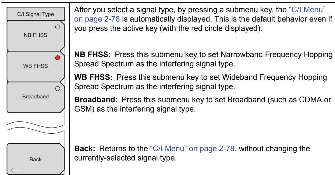
Figure 2-67. C/I Signal Type Menu
