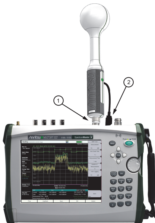
Figure 9-1. Connecting the Anritsu Isotropic Antenna
