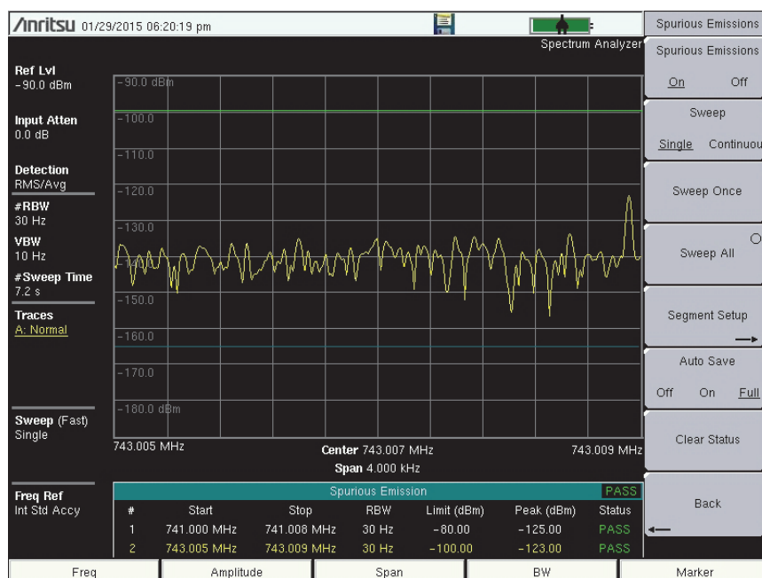
Figure 2-19. Spurious Emission Measurements
