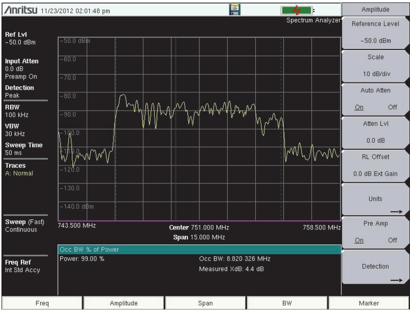
Figure 2-10. Occupied Bandwidth Results Using the % of Power Method
