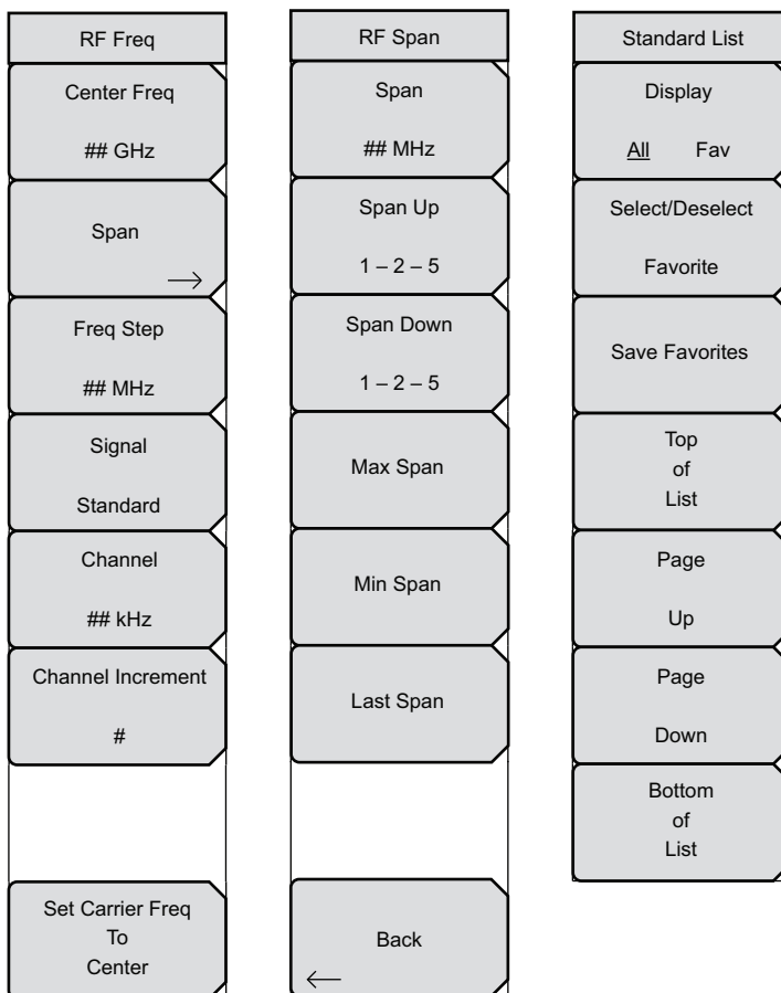
Figure 7-6. Frequency Menus with AM/FM/PM Analyzer (Option 509)
