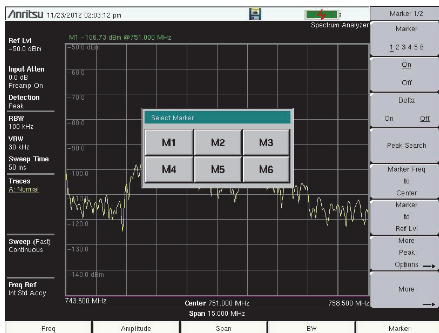
Figure 2-11. Select Active Marker with the Touch Screen
