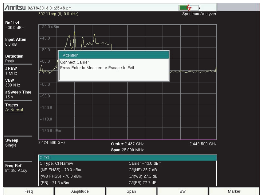
Figure 2-13. C/I Measurement, Ready to Measure the Carrier
