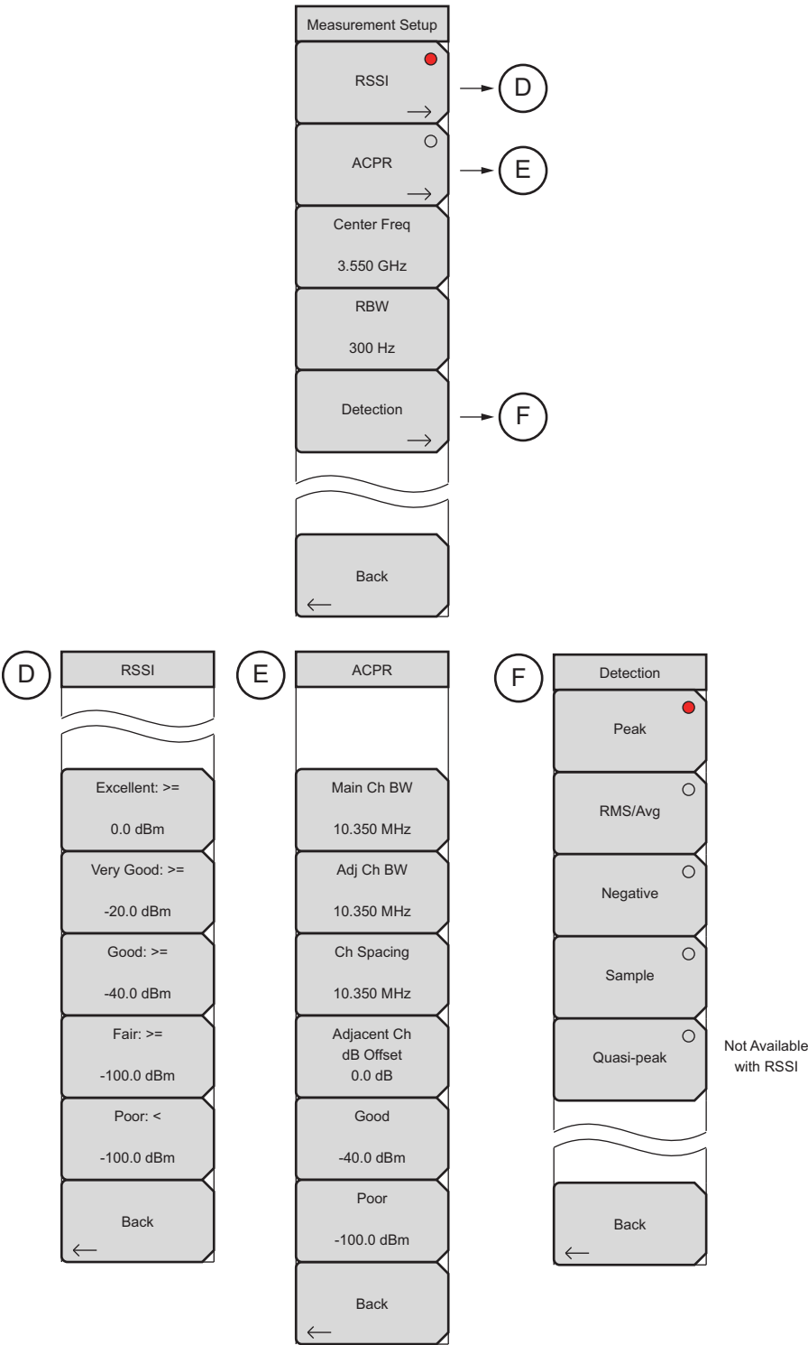
Figure 6-8. Coverage Mapping Menu Keys (Part 2)
