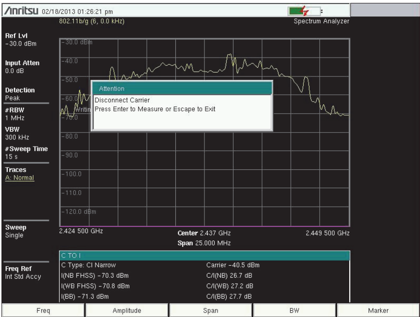
Figure 2-14. C/I Measurement, Carrier Measured
