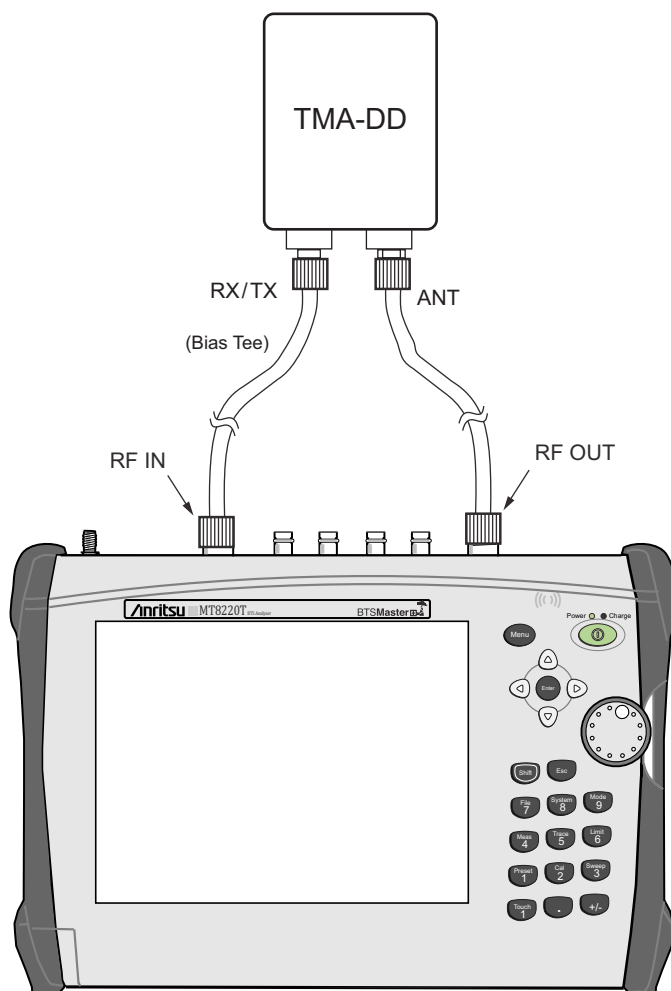
Figure 8-1. Variable Bias Tee
