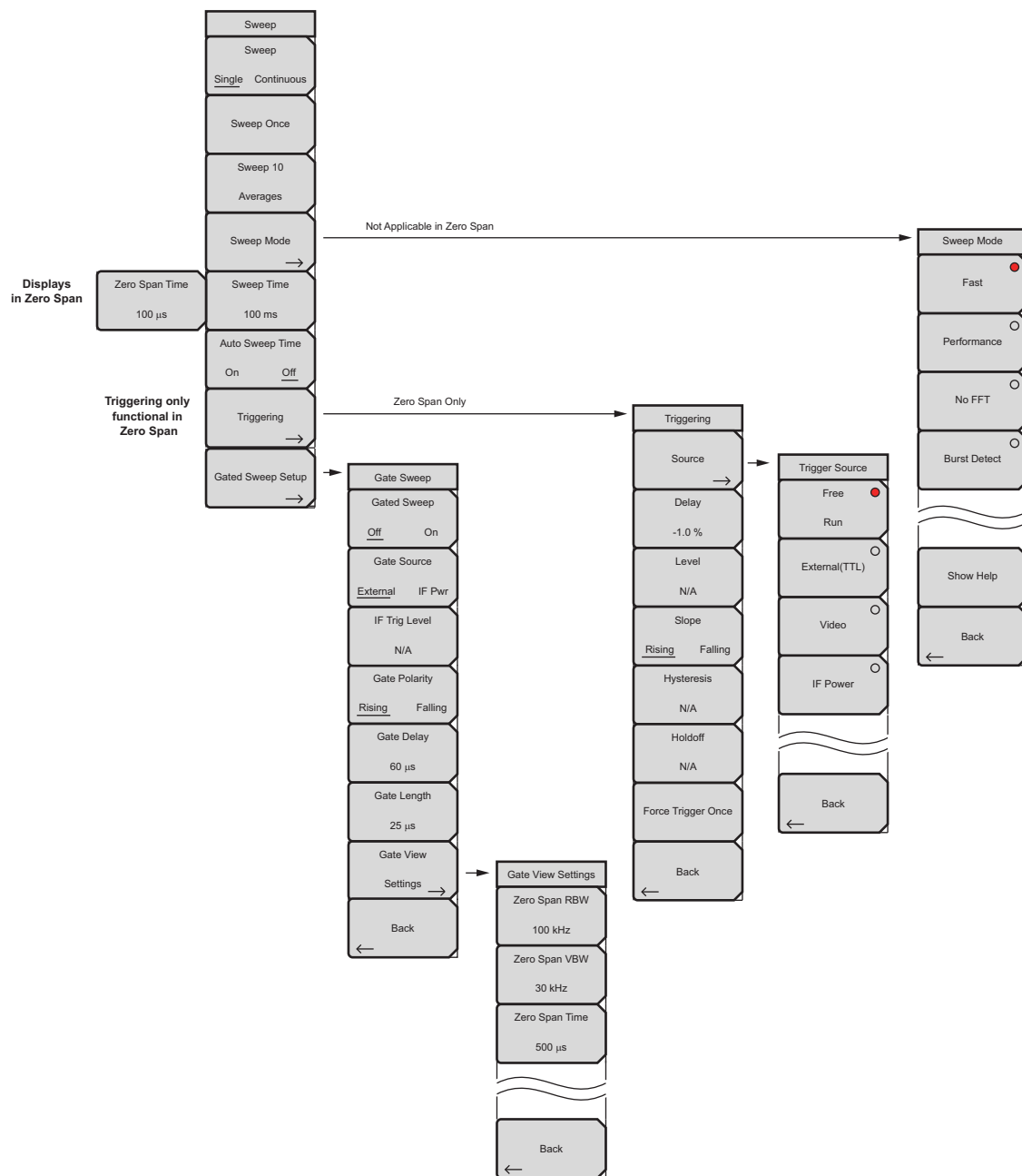
Figure 2-31. Sweep Submenu Keys
