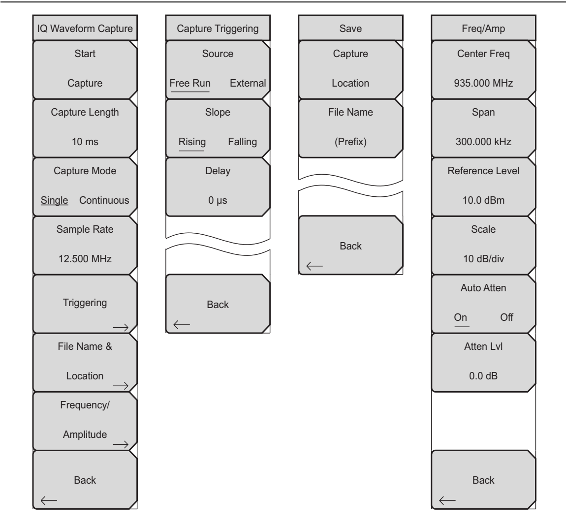
Figure 3-18. IQ Waveform Capture Submenu Keys (Option 24)
