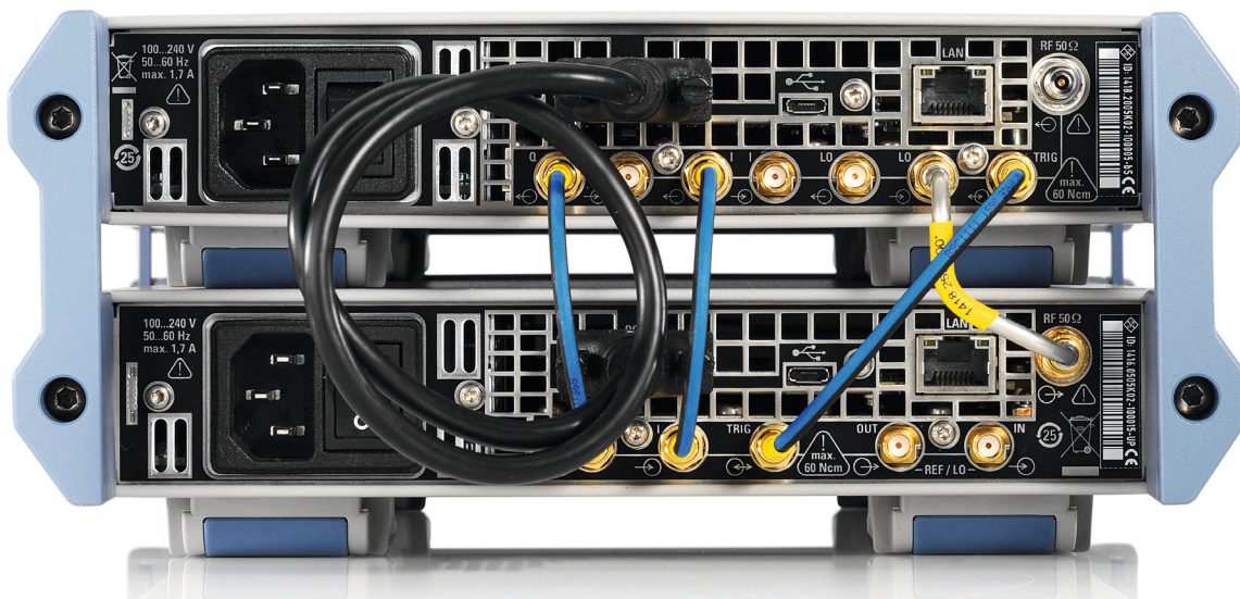
Connections between the R&S®SGS100A and the R&S®SGU100A.
