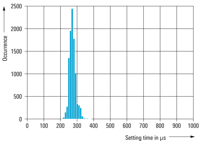
Histogram of 10 000 frequency setting times measured via PCIe interface, Setting Characteristic: AUTO, R&S®SGS100A alone
