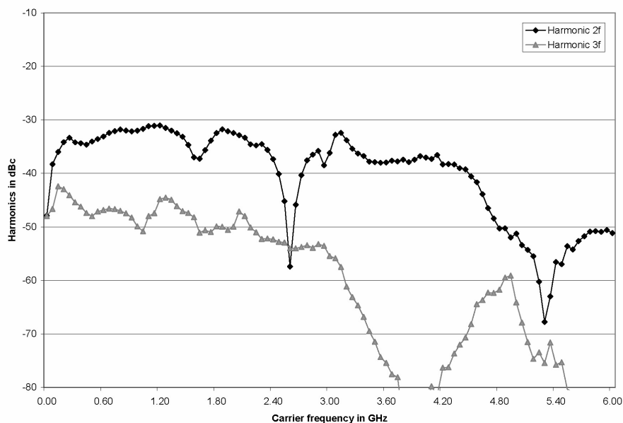
Measured harmonics at +18 dBm versus frequency
