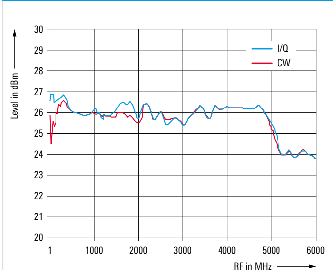
Measured maximum output power vs. frequency
